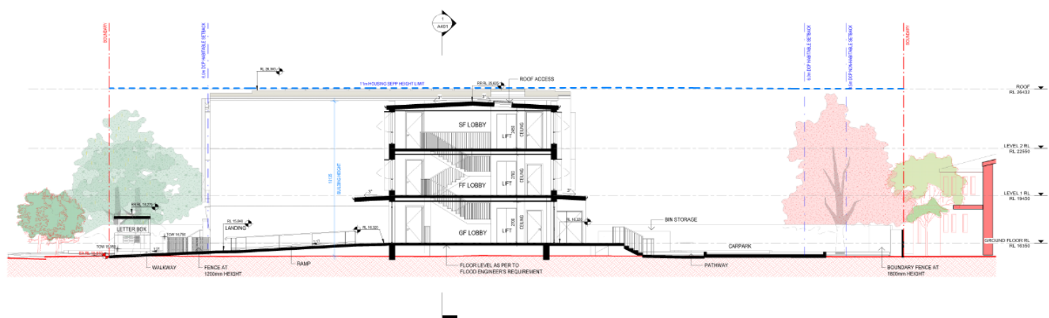
2 SHORT SECTION 1 : 100
